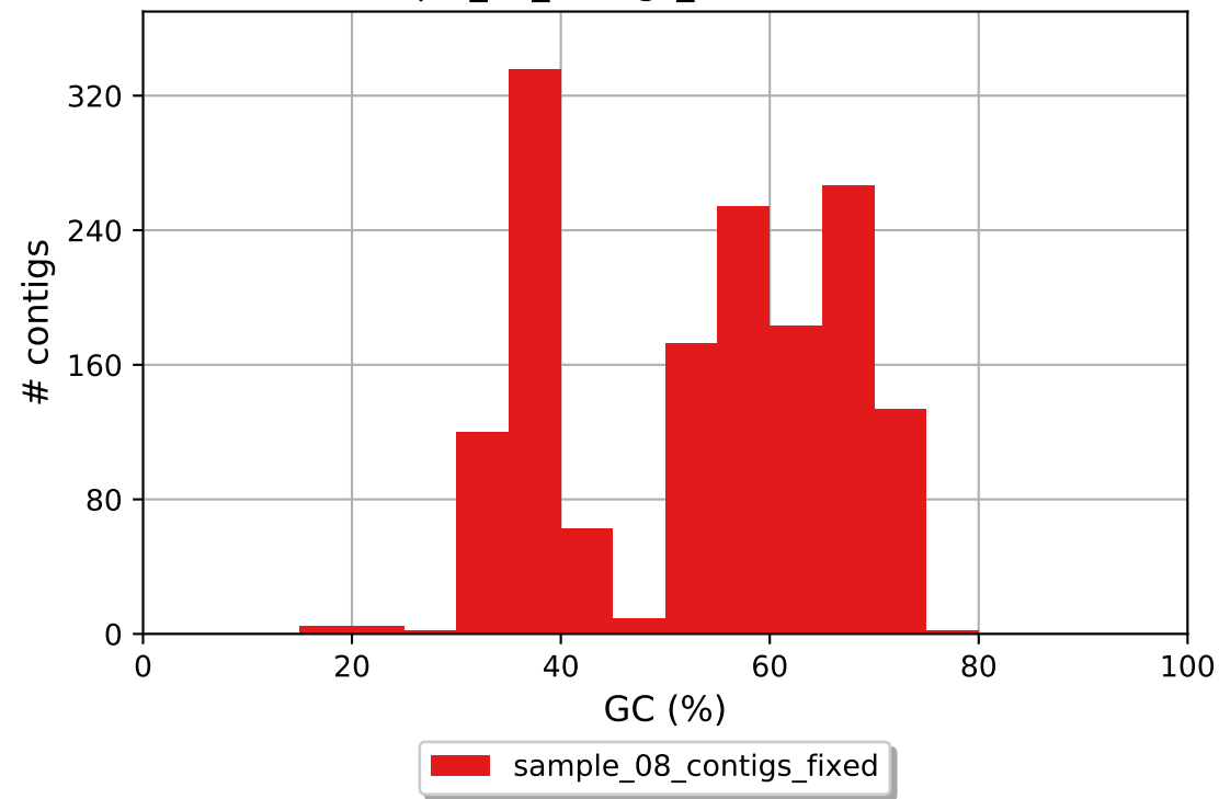
sample_08_contigs_fixed GC content
