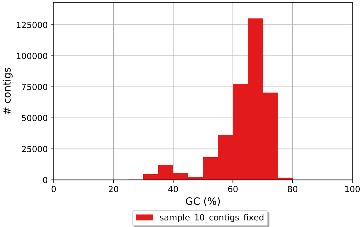
sample_10_contigs_fixed GC content
