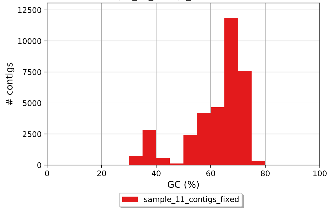
sample_11_contigs_fixed GC content
