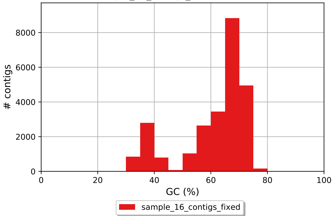
sample_16_contigs_fixed GC content
