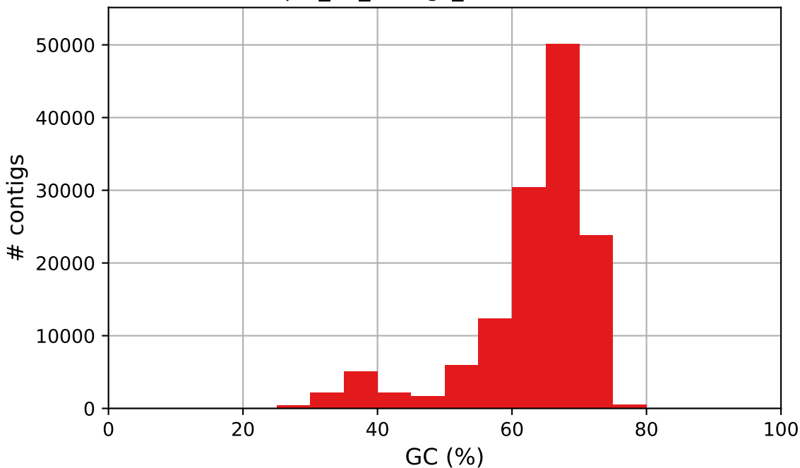
sample_17_contigs_fixed GC content
