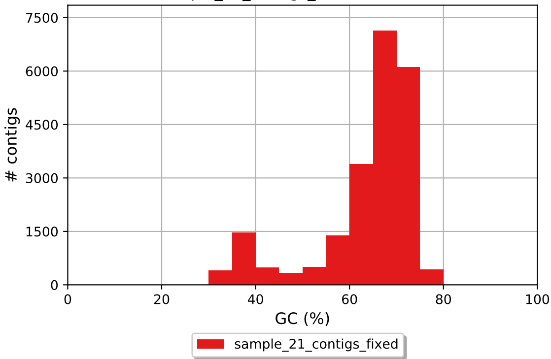
sample_21_contigs_fixed GC content
