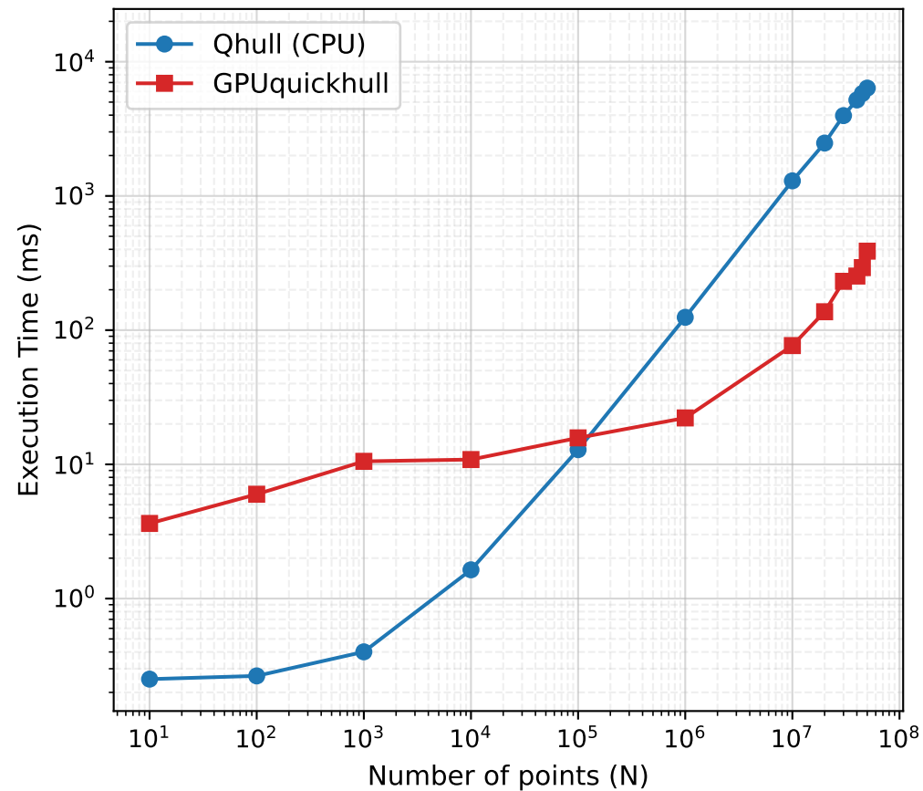
Execution Time in 2D
