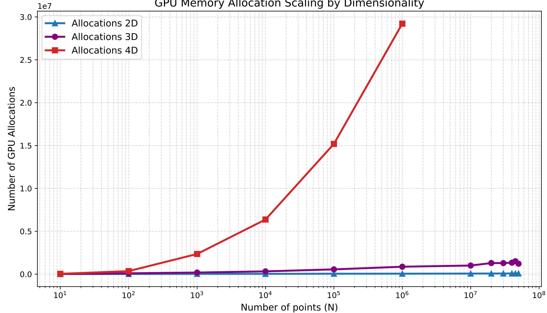
GPU Memory Allocation Scaling by Dimensionality
