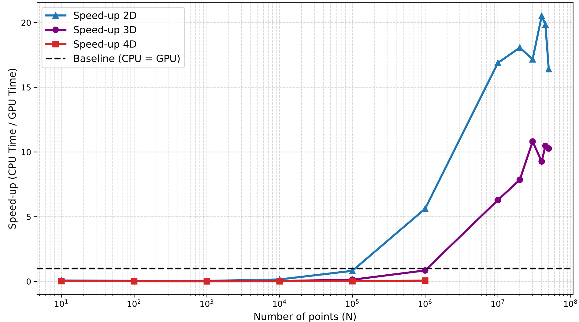
Impact of Dimensionality on GPU Acceleration
