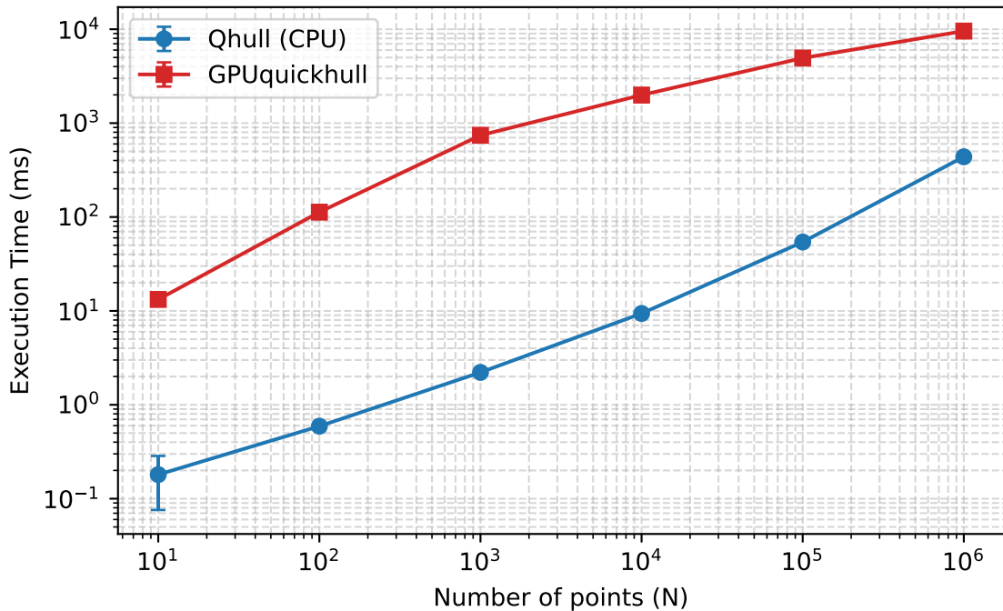
Execution Time in 4D
