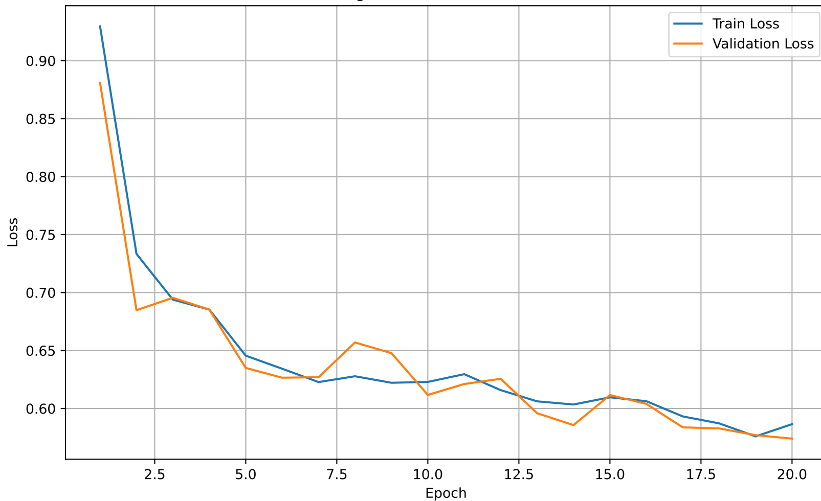
Training and Validation Loss Curves
