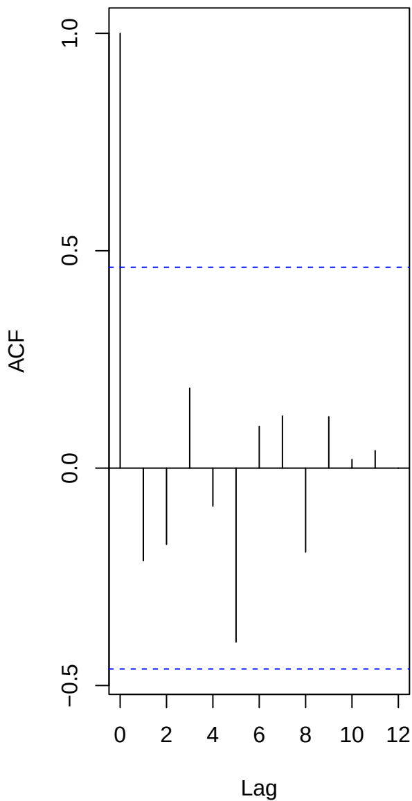
ACF – Regional M7_av
