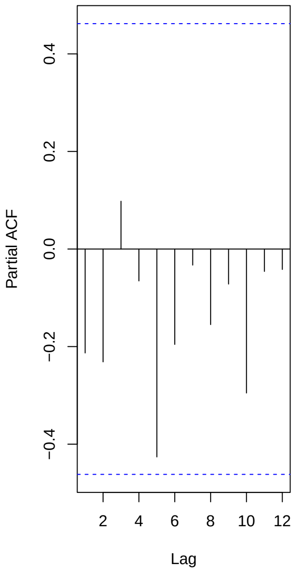
PACF – Regional M7_av
