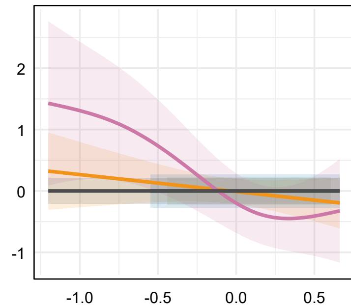
Rate of Change ( \delta T^{\circ}\text{C} / 100\text{yr} )
