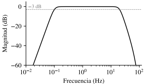
(a) Pasa banda Butterworth, orden 4 (0.1–20 Hz)
