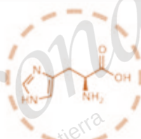
Histidina
