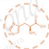
Histidina
