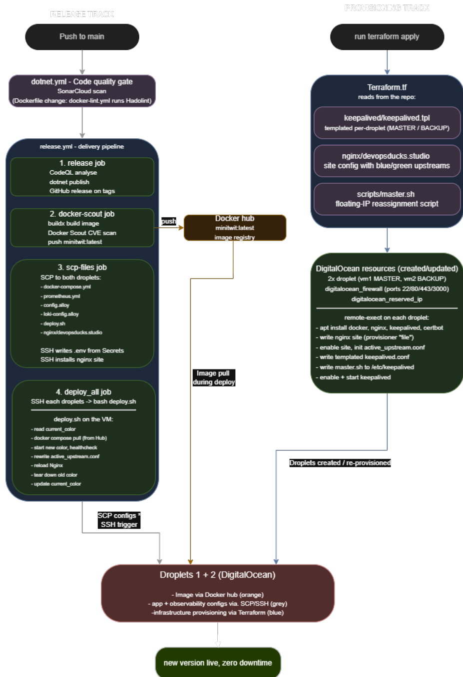
Figure 4: CI/CD Pipeline
