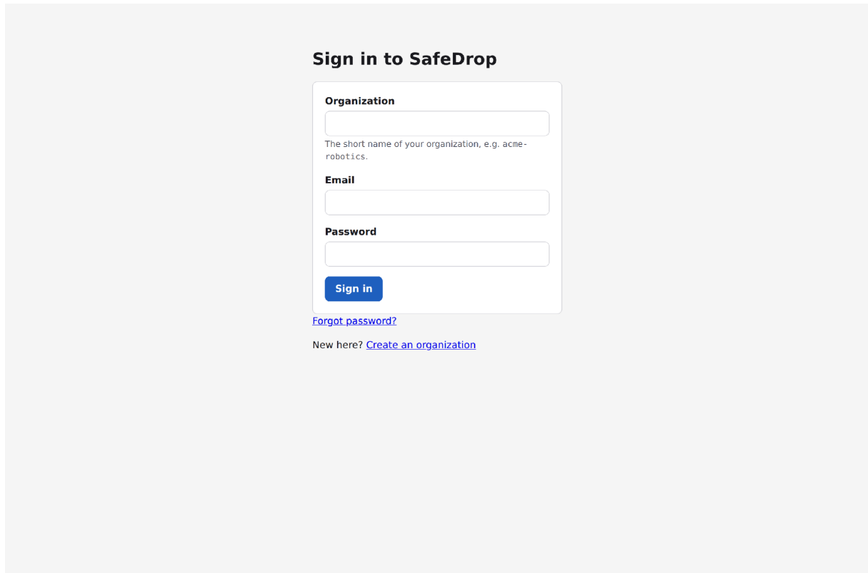
Figure 6. Sign in. The organization slug is part of the credential because email is unique per organization, not across SafeDrop (OD-3).
