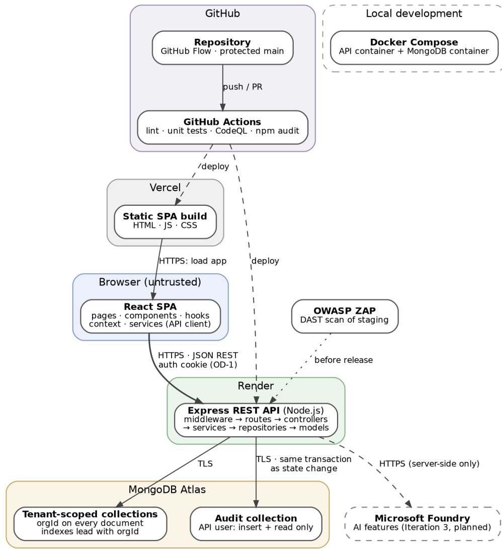
Figure 1. SafeDrop system architecture. Solid arrows are runtime traffic; dashed arrows are deployment or planned integrations; the dotted arrow is security testing.
