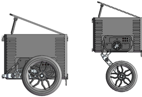
Figure 1. Intelligent logistics delivery robot wheel leg diagram.
