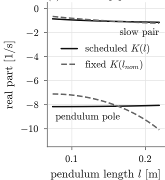
(c) closed-loop poles
