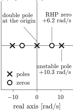
(a) open-loop poles and zeros
