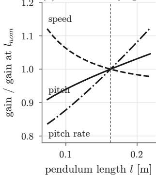
(b) scheduled LQR gains
