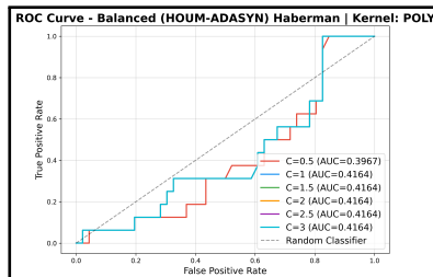
(c) Kernel Polynomial
