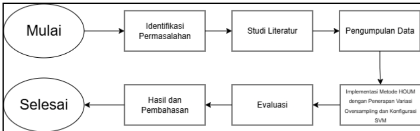
Gambar 3.1 Alur Penelitian
