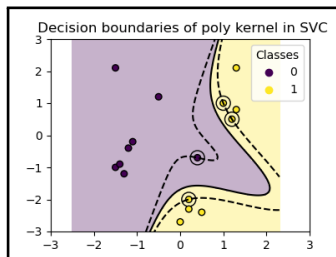
(c) Kernel Polynomial
