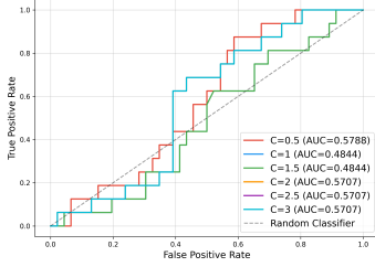
(a) Kernel Linear
