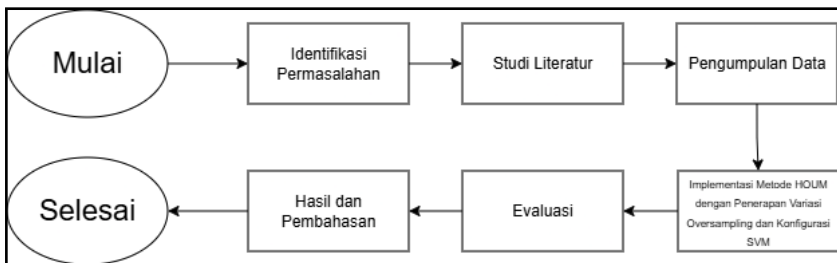
Gambar 3.1 Alur Penelitian
