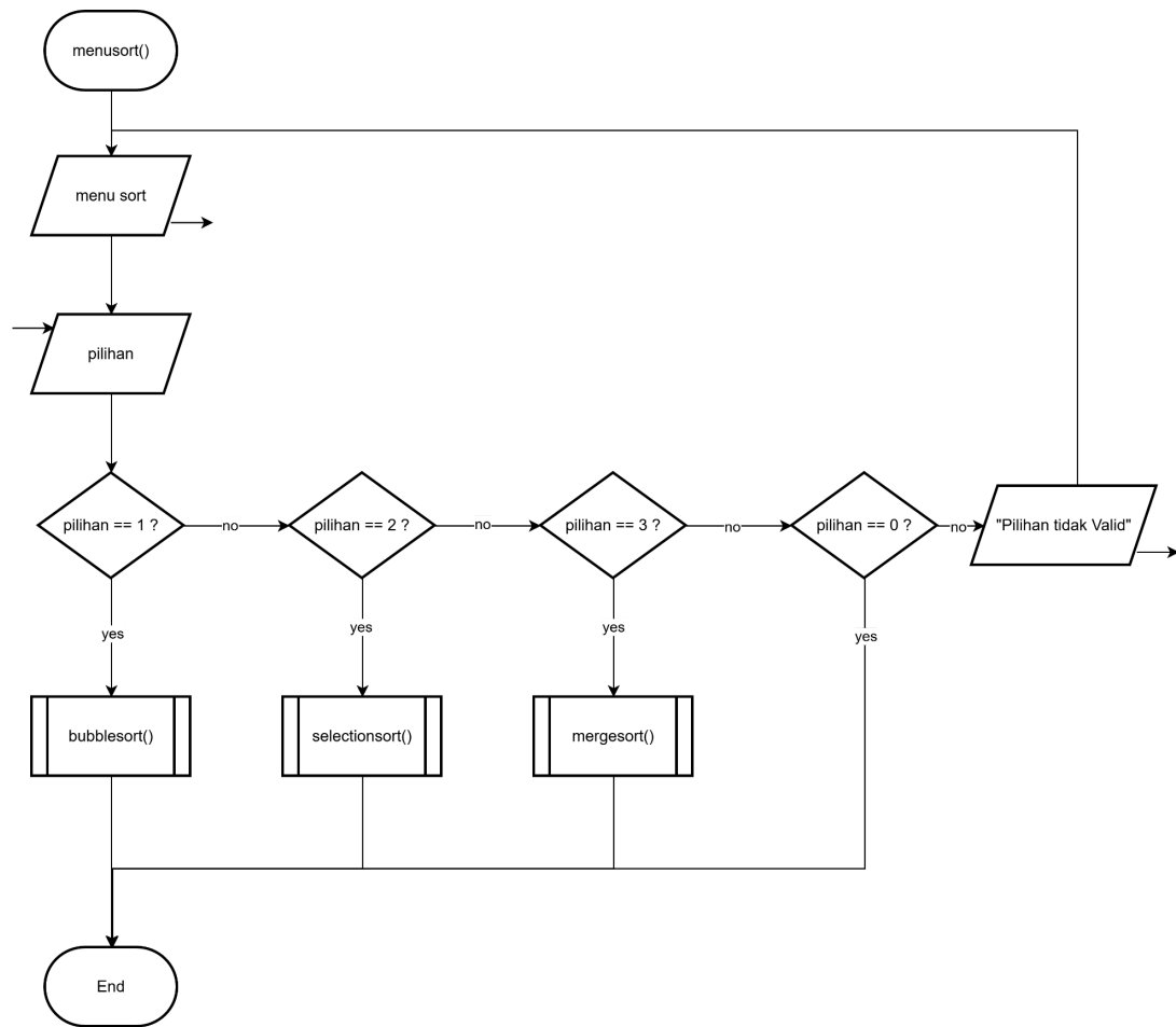
Gambar 1.6 flowchart menusort()
