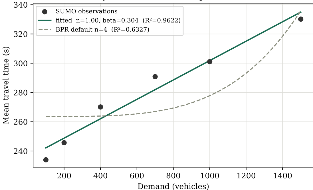
Volume-delay function calibrated against microsimulation
