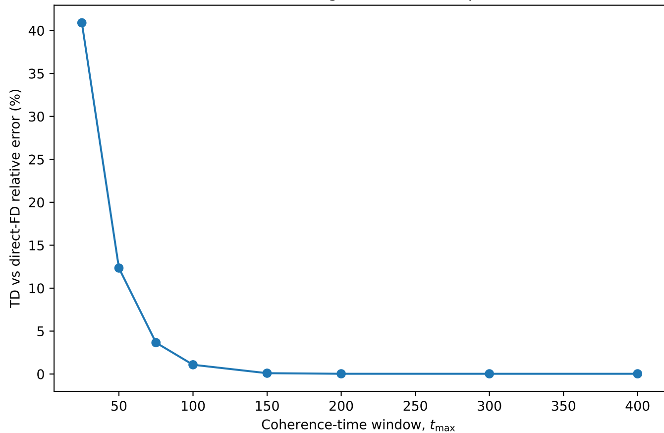
Finite-time convergence of the TD spectrum
