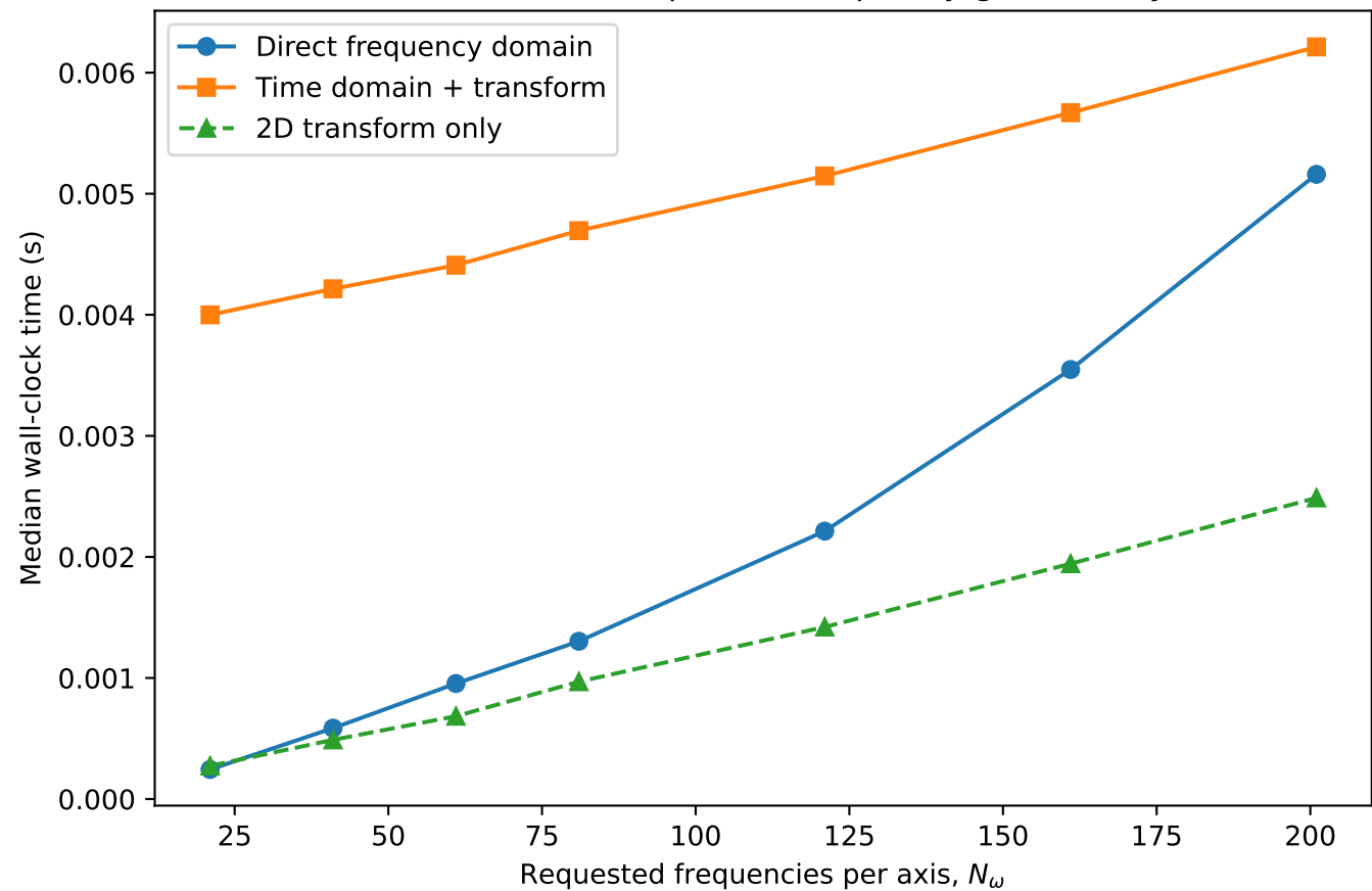
Runtime versus requested frequency-grid density
