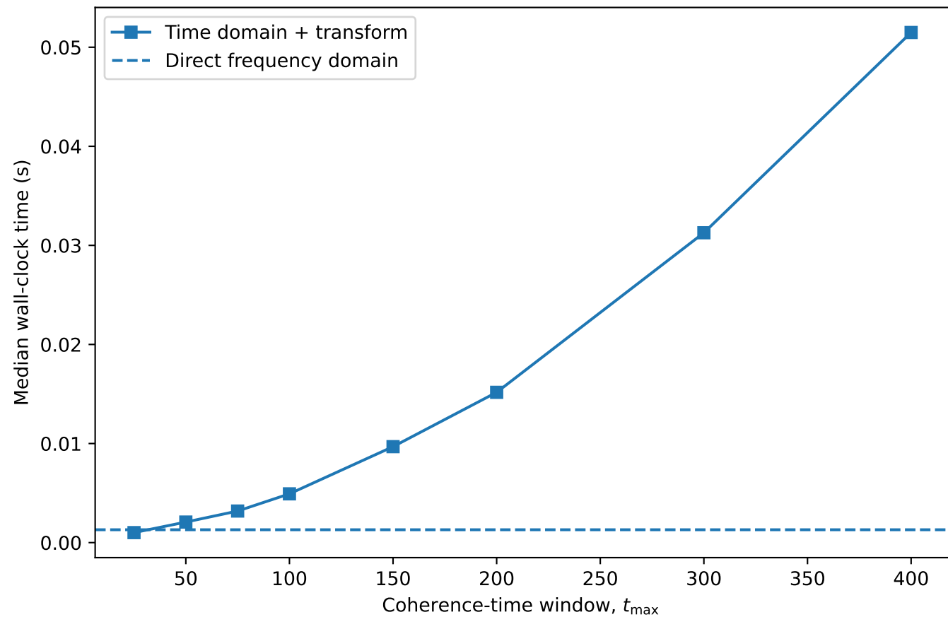
Runtime versus coherence-time window
