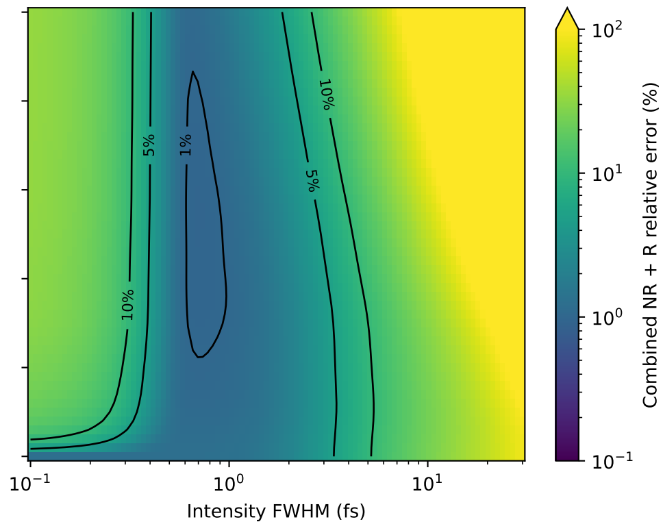
(c) Total impulsive-RWA error: A - D
