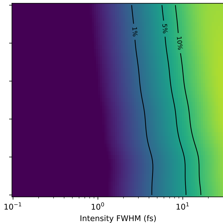
(b) In-pulse dynamics: B - C
