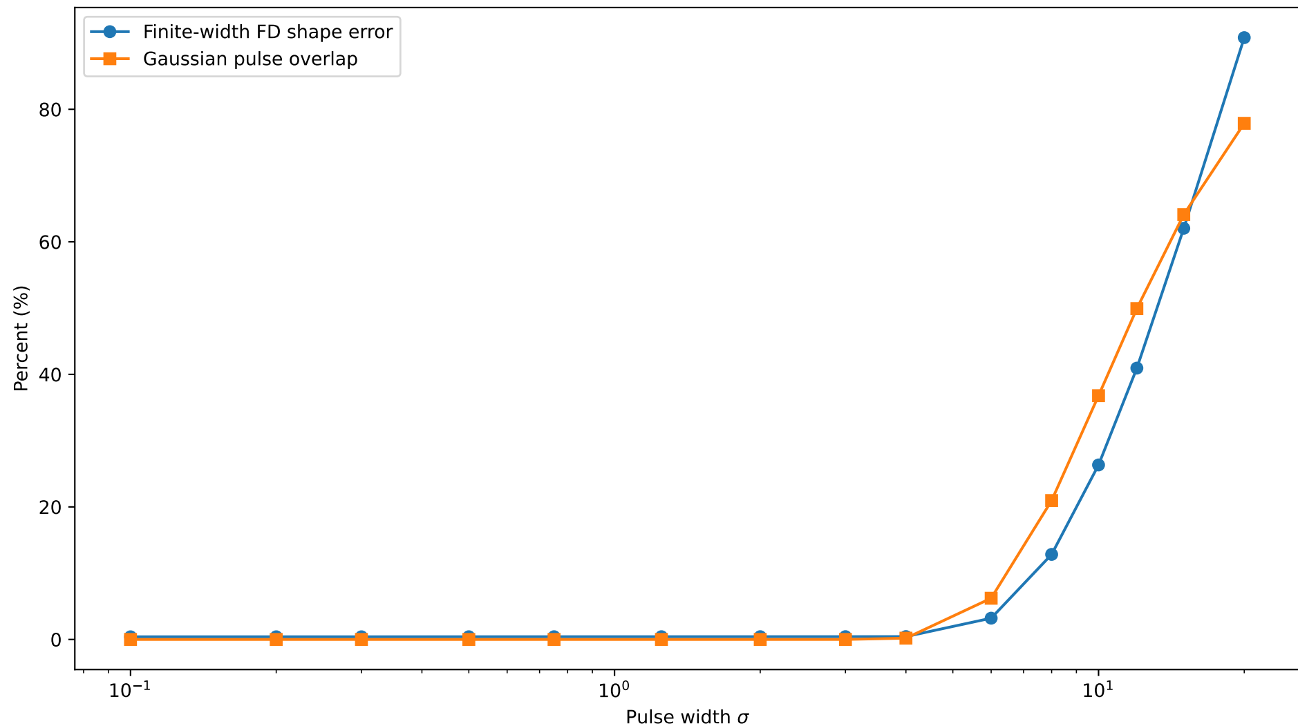
Separated-pulse FD breakdown vs Gaussian overlap, T = 20.0
