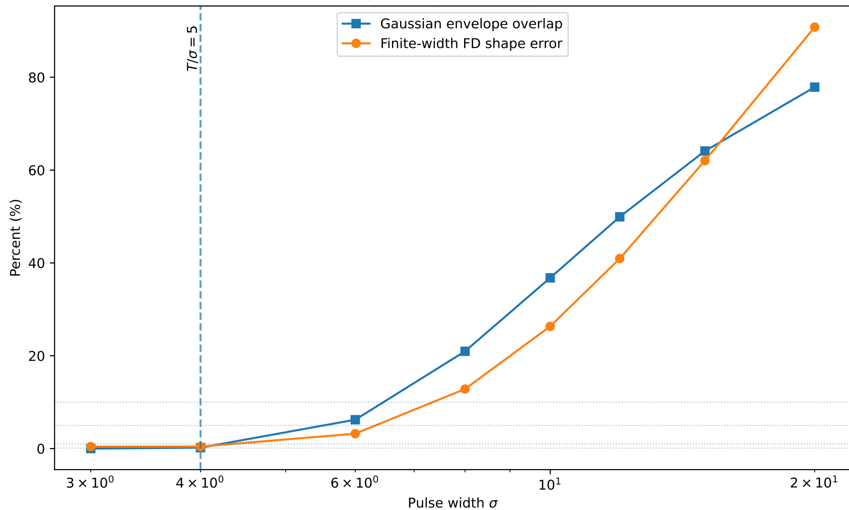
Breakdown of the separated-pulse FD approximation, T = 20.0
