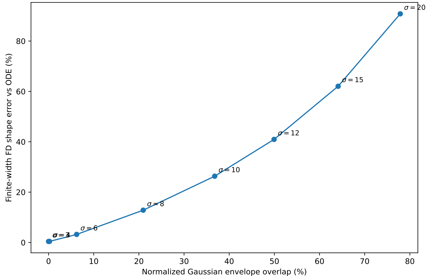
Separated-pulse FD breakdown versus pulse overlap
