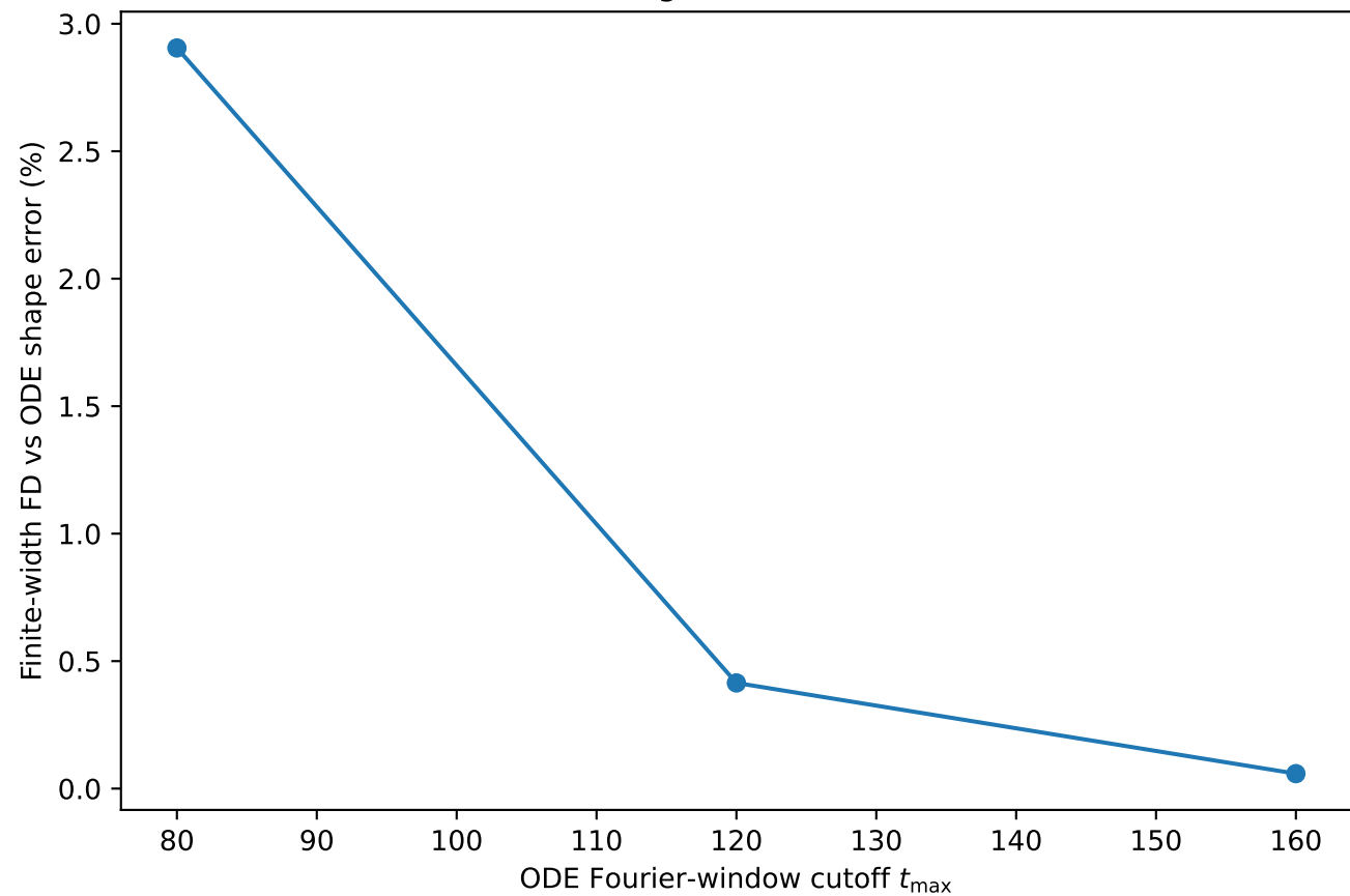
NR ODE convergence, \sigma = 1.25 , T = 20.0
