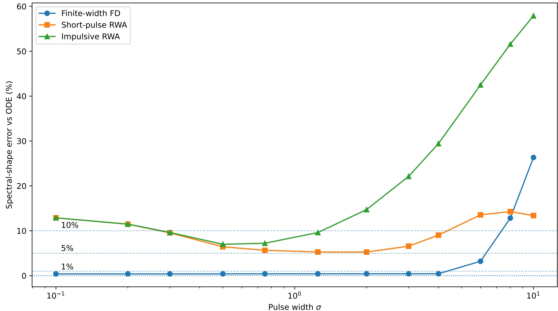
NR validity of common approximations, T = 20.0
