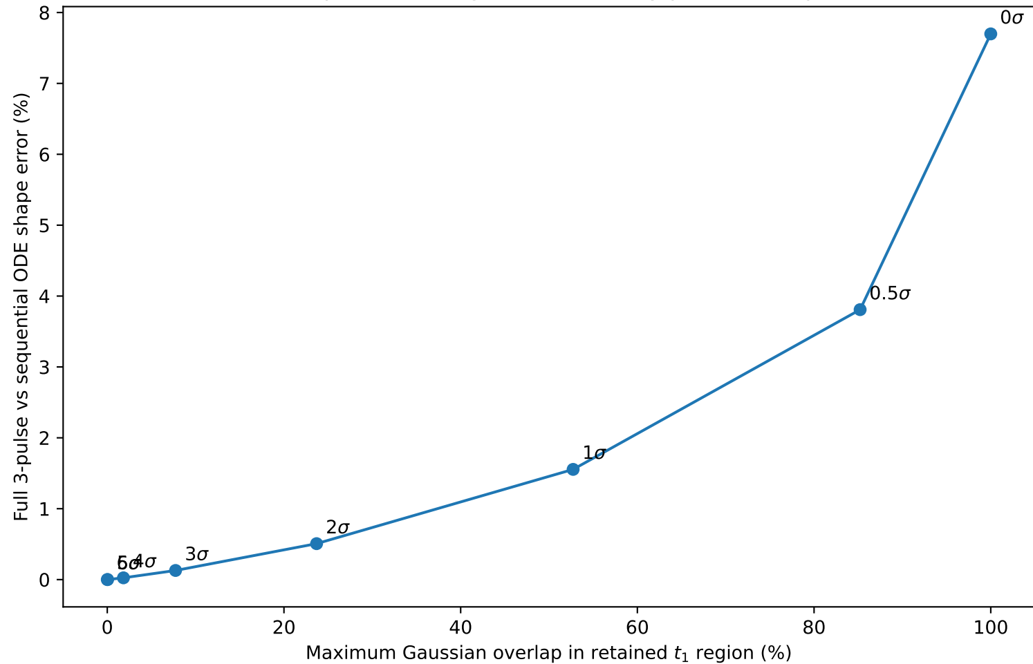
Temporal-ordering error caused by pulse overlap
