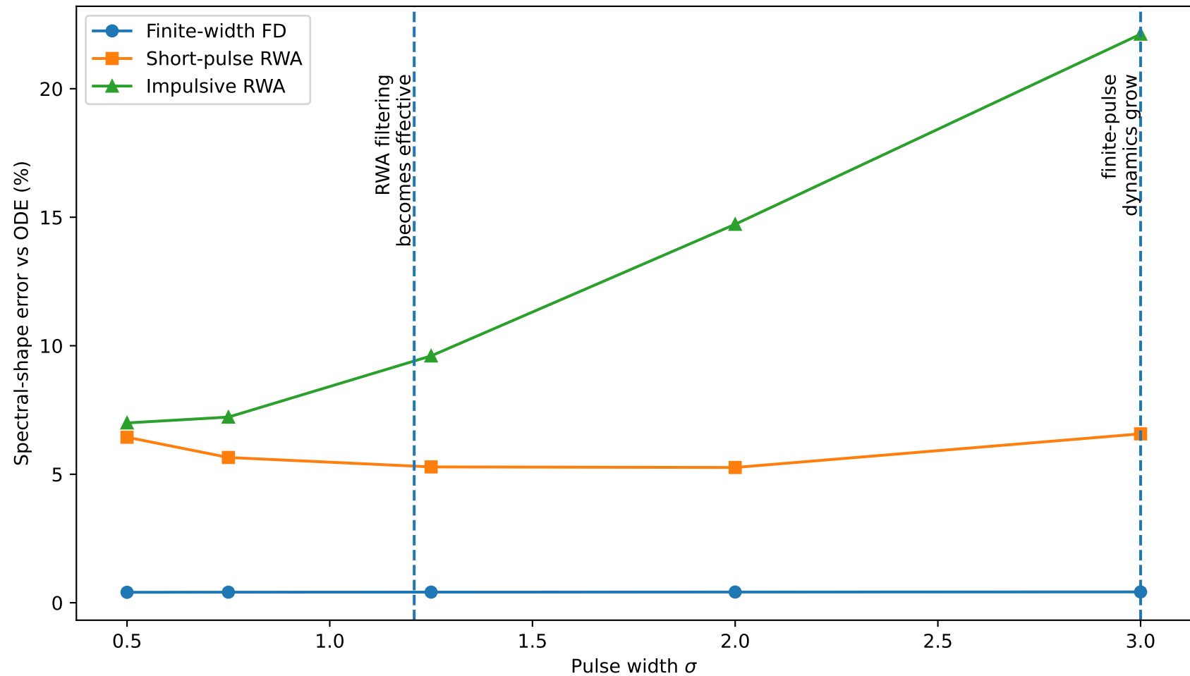
NR approximation regimes, T = 20.0
