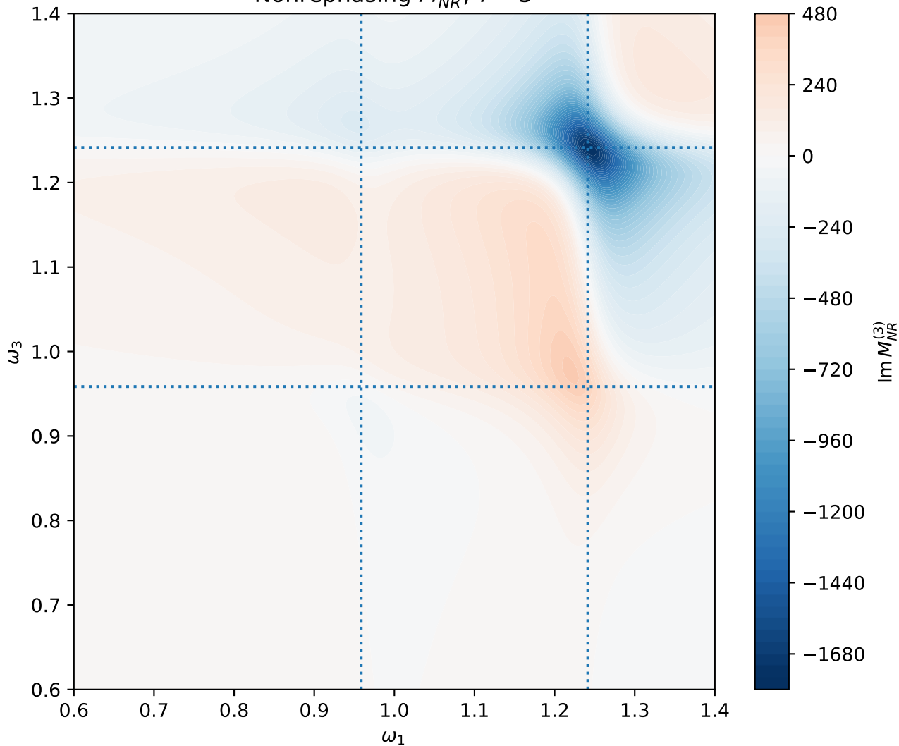
Nonrephasing M_{NR}^{(3)} , T = 5
