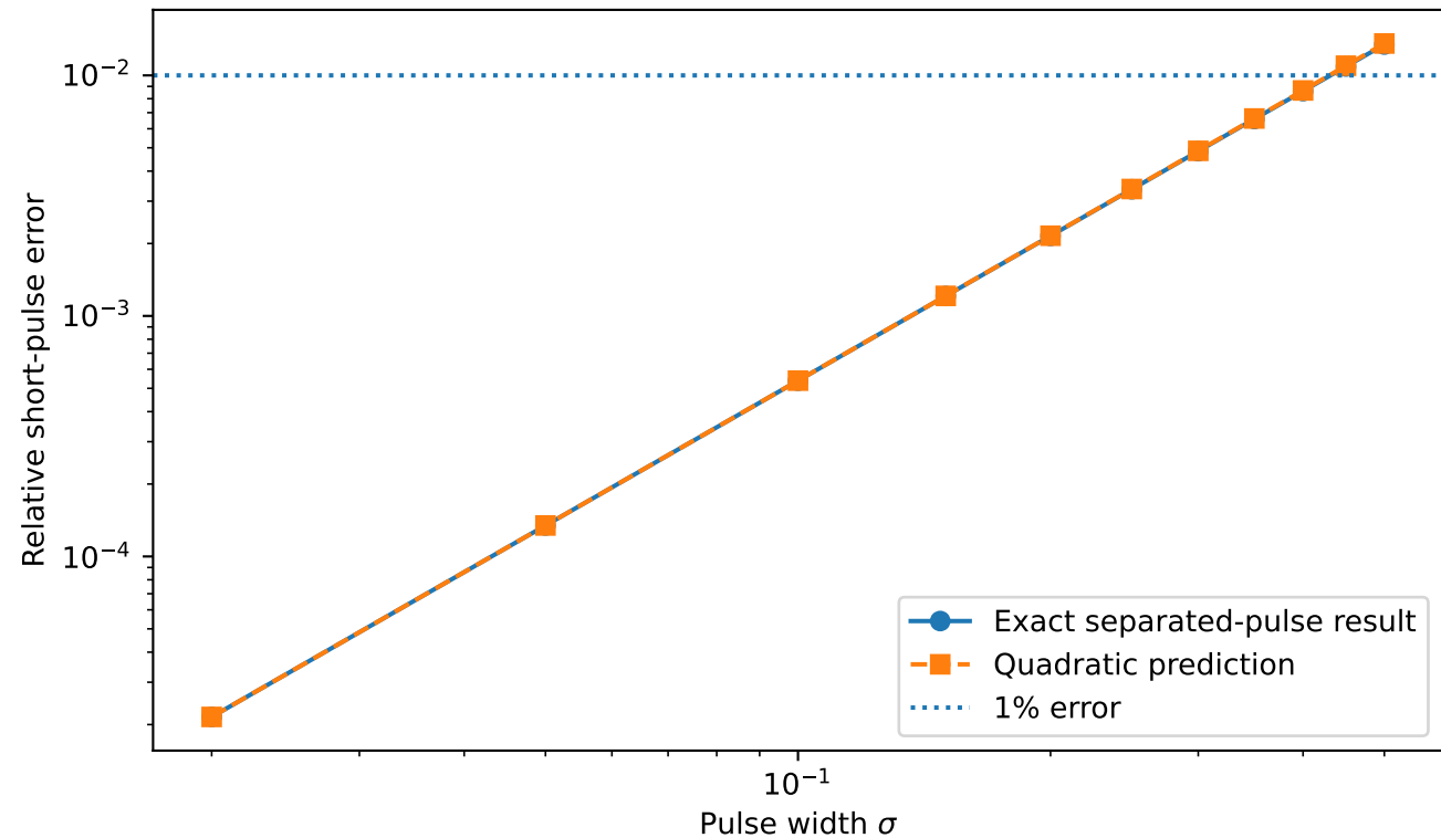
Short-pulse breakdown at (\Omega_-, \Omega_-)
