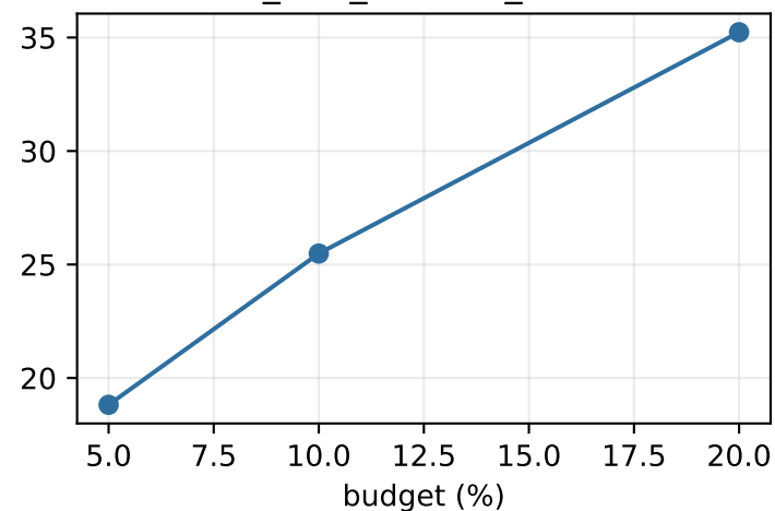
case_wall_runtime_seconds
