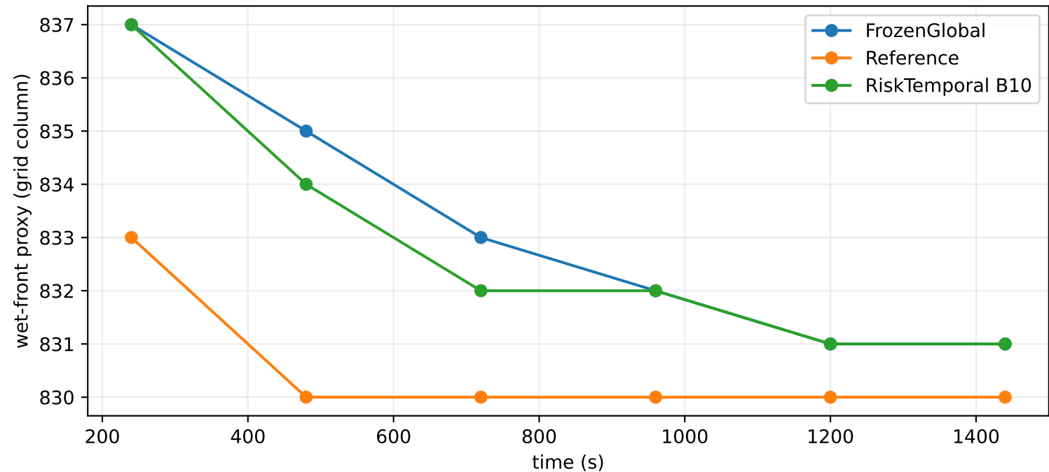
H0 propagation-front evolution
