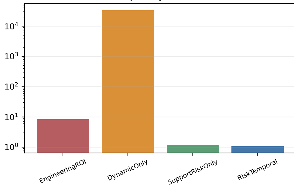
volume relative error
