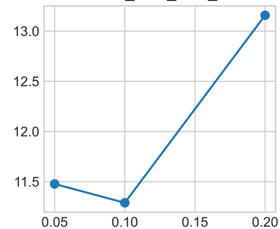
debris_front_mae_km
