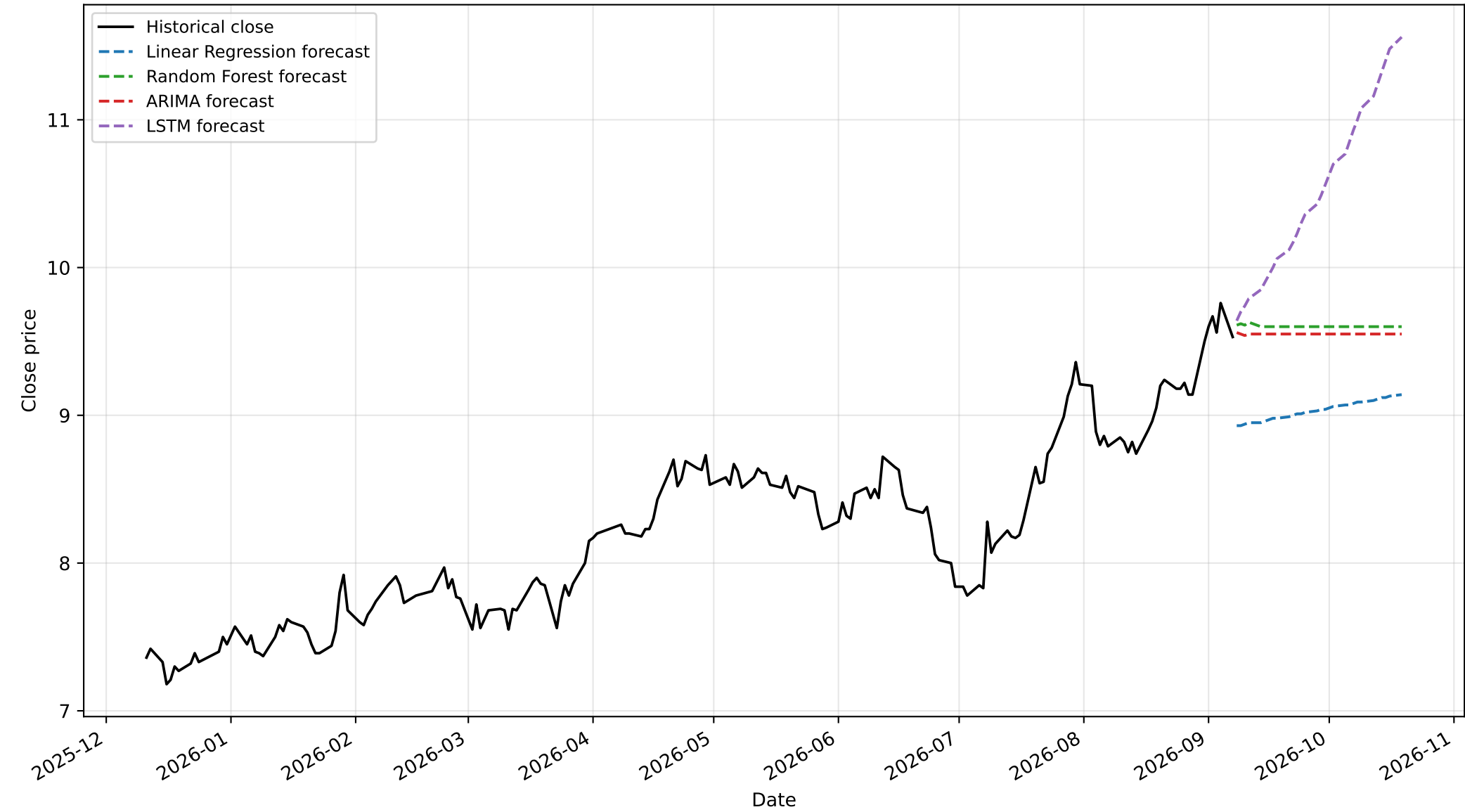
0939.HK — Historical Close and Model Forecasts
