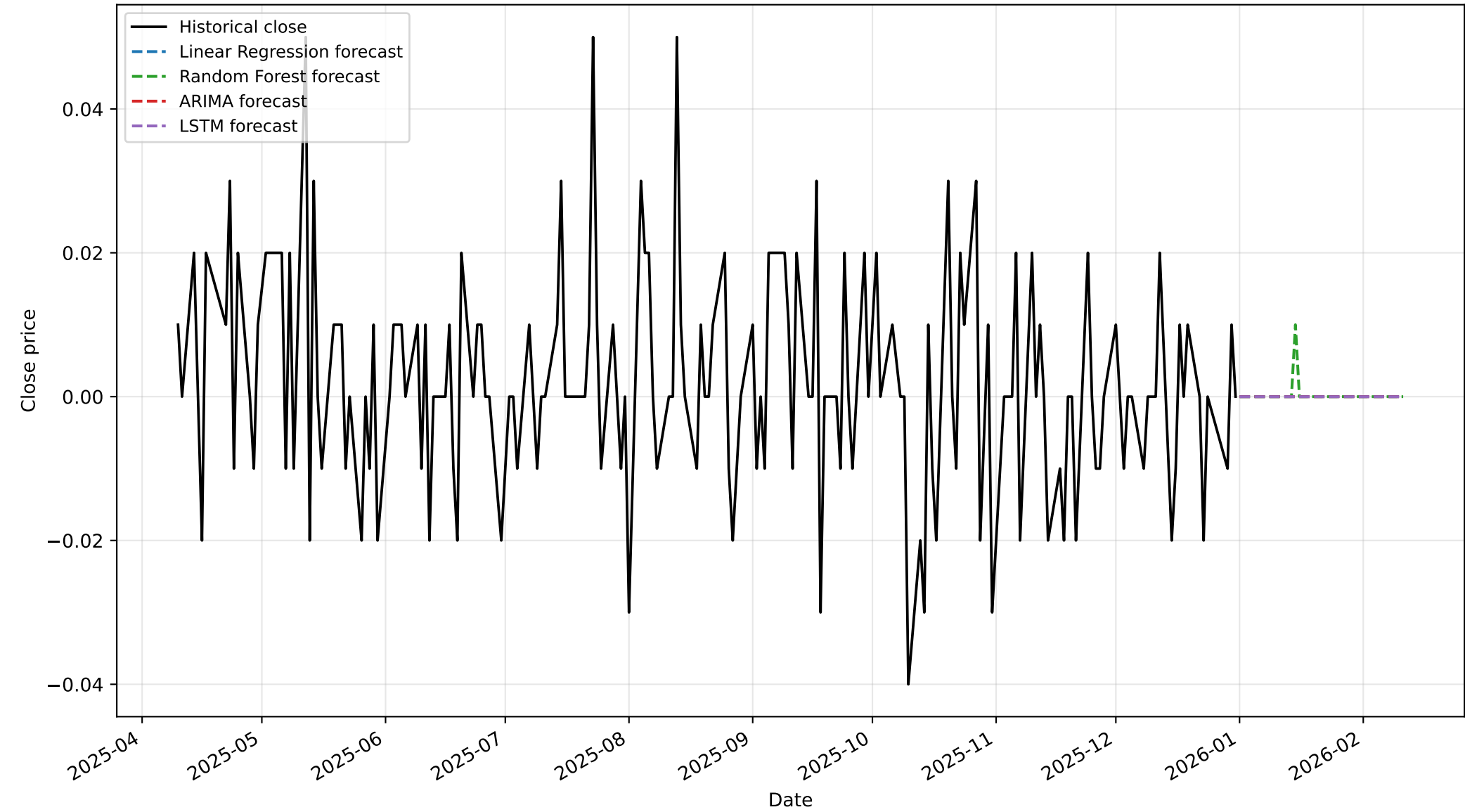
0005.HK — Historical Close and Model Forecasts
