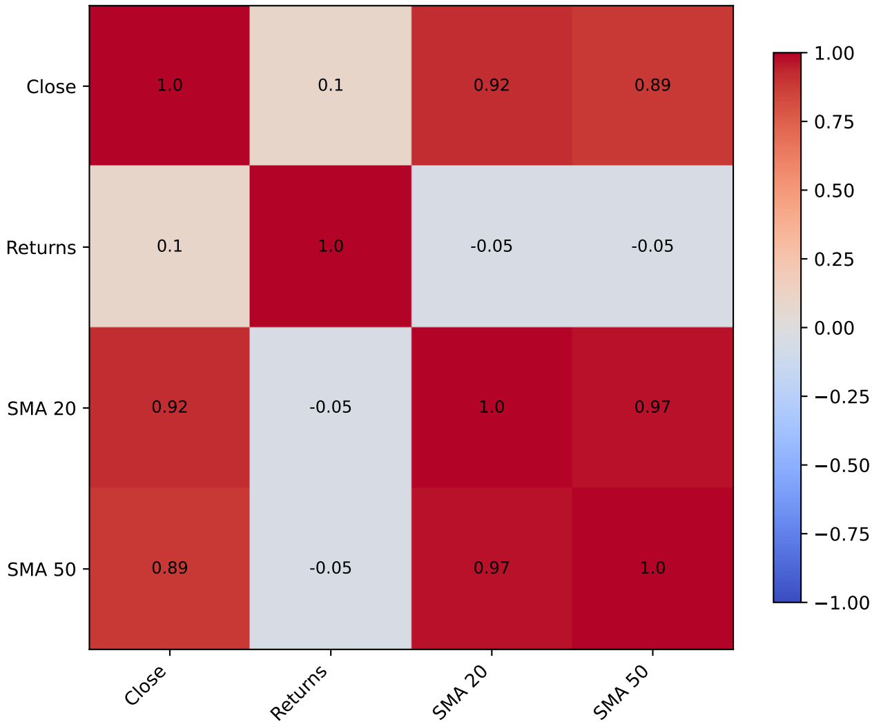
Correlation matrix
