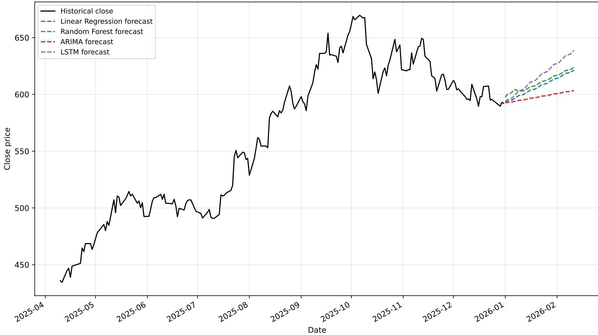
0700.HK — Historical Close and Model Forecasts
