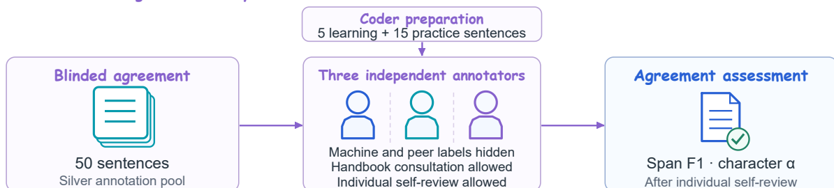
Figure 2. Human-reference construction, Silver annotation and sampled review, and the separate blinded agreement study.
