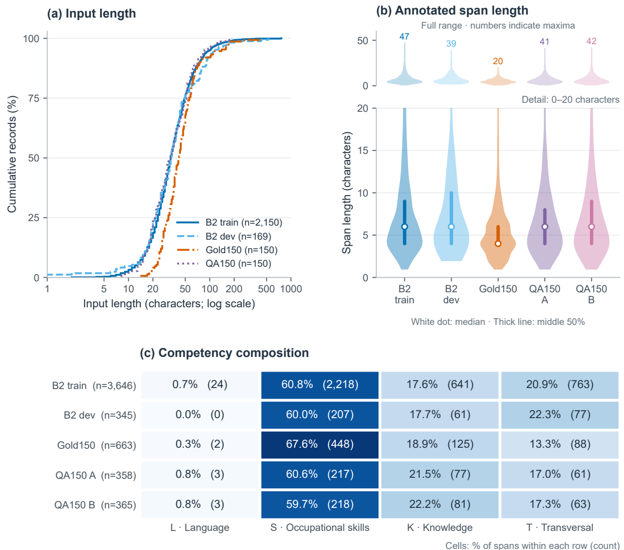
Figure 3. Benchmark annotation profile. (a) Empirical cumulative input-length distributions, including records with no spans; the horizontal axis is logarithmic. (b) Span-length violins: the main view enlarges 0–20 characters, covering 96.4–100.0% of spans in each layer; the upper overview retains the full range and labels the maxima. Both views use the same full-data density and equal maximum widths. White dots and thick lines mark medians and interquartile ranges. (c) Within-layer type percentages and span counts. B2 train/dev are the original 2,150/169-record Qwen manifests; Gold150 is the frozen 150-sentence reference. QA150 A/B are the two assisted-review layers of the same additional 150 sentences, shown once in (a). Lengths include punctuation and spaces; repeated B2 records are retained. These profiles describe historical supervision and review components; the independent three-annotator sample and the full expanded pool are not included.
