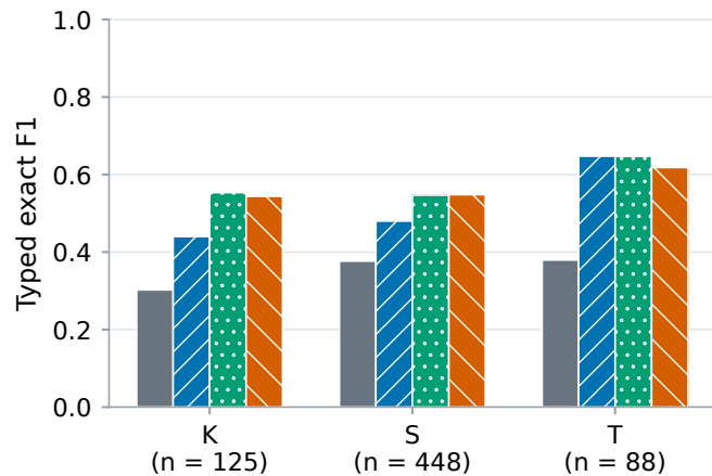
(a) F1 by competency type
